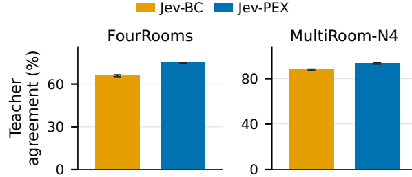
Figure 9: Teacher-action absorption at 10k. Agreement on fixed logged request states, averaged over three student seeds. Error bars show SEM.
