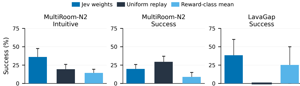
Figure 12: Sampling-weight analysis on fixed experience. Intuitive and success-oriented ratings are evaluated separately, using the same learner and original environment reward. Reward-class means preserve total preference for positive-reward transitions while removing within-class weight differences. Bars show mean \pm SEM across three seeds; each learner is evaluated on 100 episodes.
