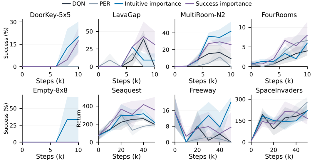
Figure 8: Replay-sampling learning curves on the selected tasks, mean \pm SEM.
