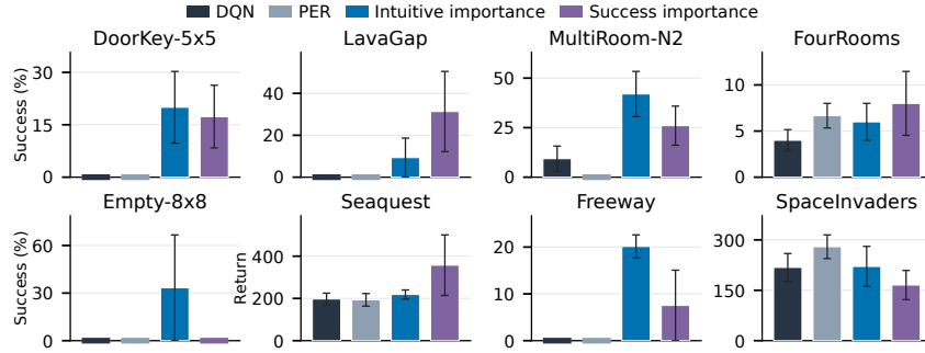
Figure 5: RL with Jev-Rewighted Replay. MiniGrid 10k and Atari 50k endpoints, mean±SEM across three training seeds. Tasks with zero performance for all four methods are omitted.
