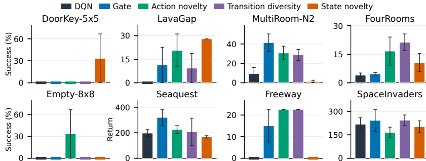
Figure 4: RL with Jev Exploration. MiniGrid 10k and Atari 50k endpoints, mean±SEM across three training seeds. Tasks with zero performance for all four methods are omitted.
