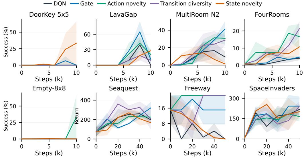
Figure 7: Exploration learning curves on the selected tasks, mean \pm SEM. Curves end at their last available common evaluation node.
