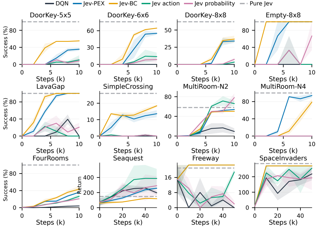
Figure 6: Reference-method learning curves, mean \pm SEM. The horizontal dashed line is the independently evaluated pure-Jev policy; it has no training-step dependence.
