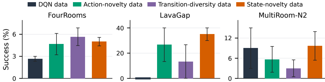
Figure 10: Data quality separated from shaping. All learners use only environment reward on their respective fixed 10k experience streams, with matched learner settings and sampling indices. Evaluation uses 100 environment seeds; bars show mean \pm SEM over three data/training seeds.
