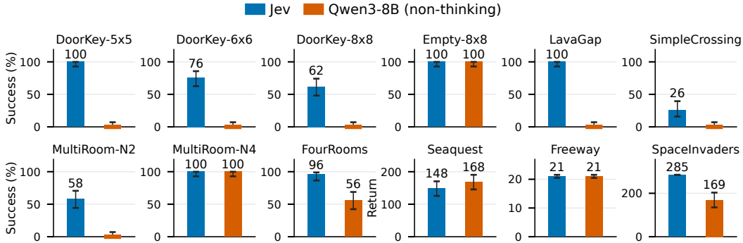
Figure 2: Direct control with matched structured inputs. Jev and non-thinking Qwen3-8B use the same evaluation seeds and task-specific input construction. MiniGrid: success on 50 episodes with 95% Wilson intervals. Atari: mean native return over five complete games with SEM. A colored horizontal stroke denotes zero successes. FourRooms and MultiRoom-N4 use the full-navigation input; the other tasks use their direct-Jev input interface.
