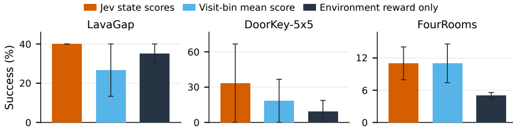
Figure 11: State-dependent reward information on fixed experience. The bin-mean control replaces scores with their average within 2k-step collection windows and visitation bins. Original and bin-mean scores have matched overall means but different fine-grained allocations. Bars show mean \pm SEM across three seeds; each fitted learner is evaluated on 100 episodes.
