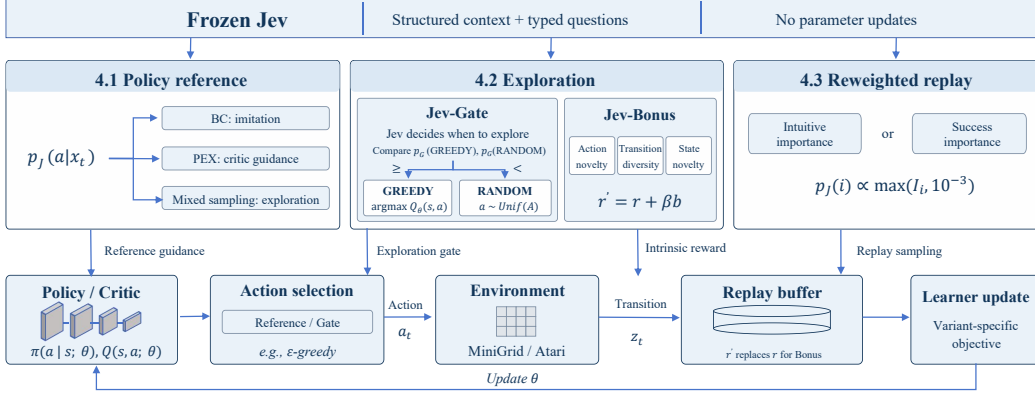
Figure 1: The framework structure of Jev for RL.
