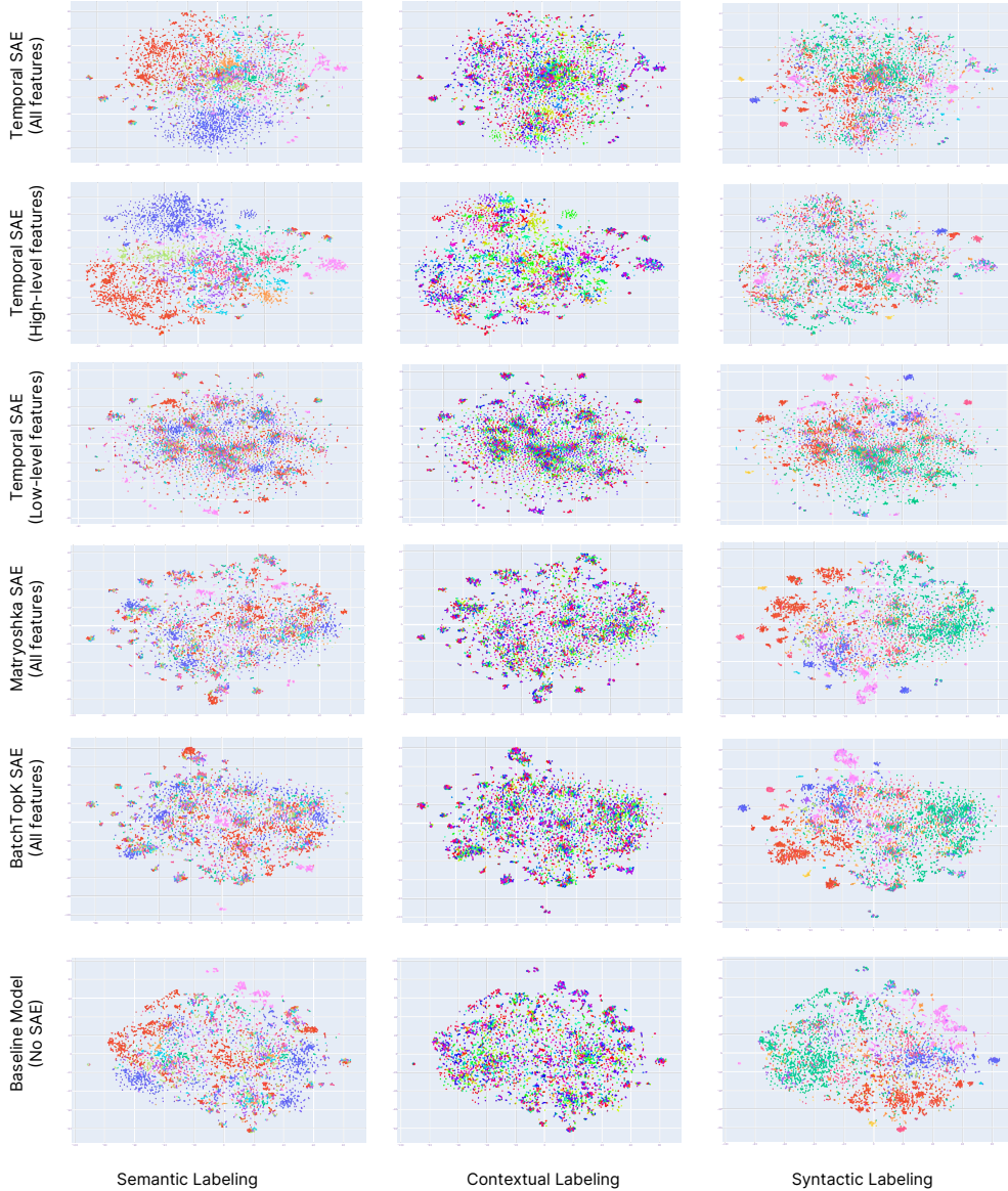
Figure 12: TSNE visualizations of Pythia-160m SAE decompositions of MMLU questions, labeled by question category (left), question number (middle column), and token part of speech (right). We see that the high-level features from Temporal SAEs (second row) recover semantic and contextual information. The low-level features of Temporal SAEs (third row), as well as Matryoshka and BatchTopK SAEs (fourth and fifth row), recover syntactic information. Baseline model latent (last row) balance a mix of information.
