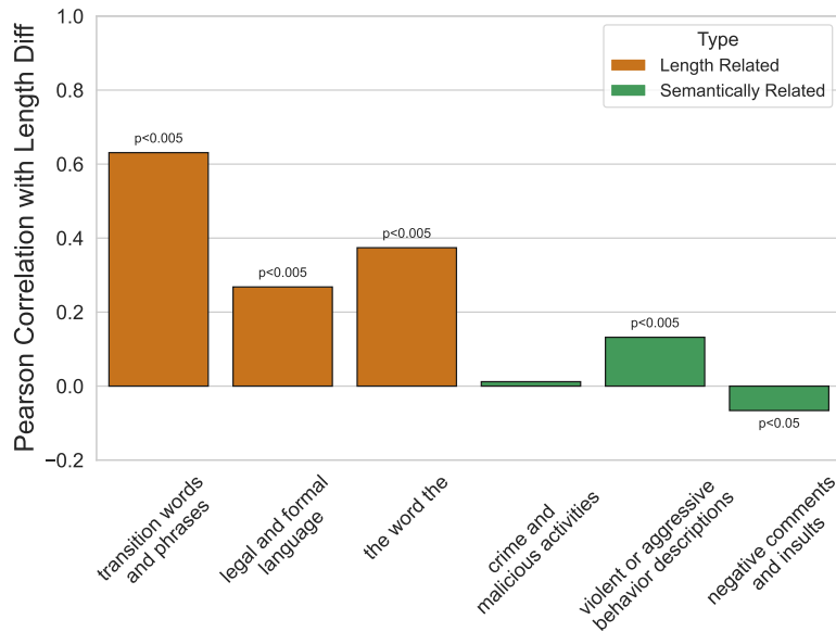
Figure 6: Correlation of difference in T-SAE feature activations (rejected—chosen) with difference in response length (rejected—chosen). Selected features all have high difference in feature activations between chosen and rejected completions (selected from top 15), yet semantically-relevant features are less correlated with length difference while spurious features are more correlated.
