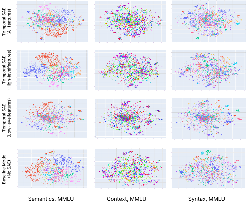
Figure 9: TSNE results for T-SAE trained on Llama-3.1-8b-Instruct
