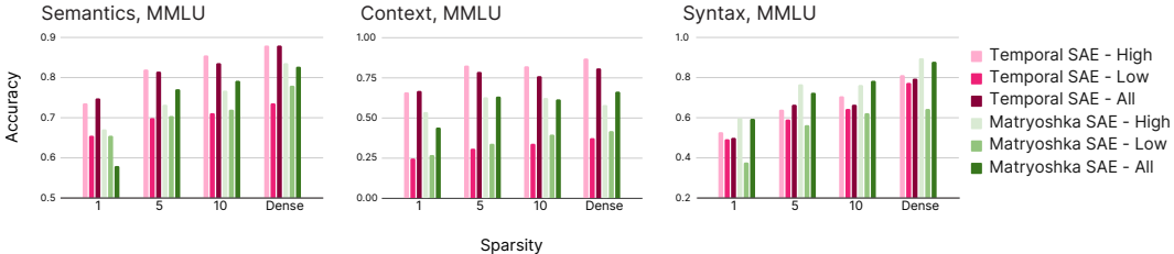
Figure 7: Probing results split across high and low splits for Temporal and Matryoshka SAEs.
