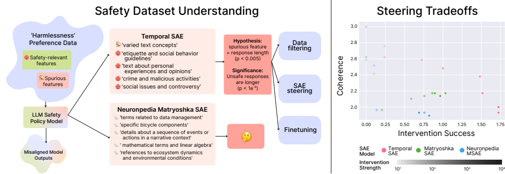
Figure 5: Left. We use SAEs to understand user preferences in the HH-RLHF Bai et al. (2022) dataset. The Matryoshka SAE appears to find more random features, whereas the T-SAE is able to capture safety-relevant features. The T-SAE also finds a spurious length correlation in the dataset, where rejected completions are longer than chosen completions. Right. We find that high-level features Pareto dominate baselines in their ability to steer LLMs. Specifically, they are better at preserving coherence while successfully changing the semantics of model generation.
