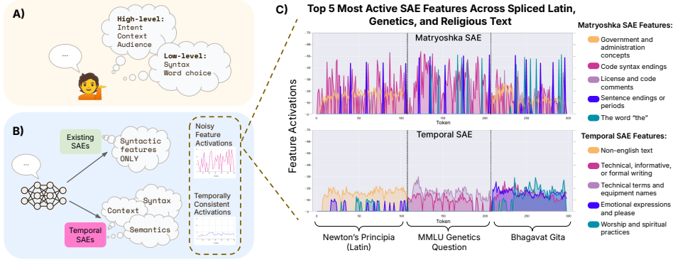
Figure 1: A) Human language production involves high-level features such as semantic content and surrounding context, as well as low-level features such as syntactical requirements and specific word choices. B) While existing SAEs mostly recover syntactic information, T-SAEs balance recovery of semantics, syntax, and context. C) When decomposing a sequence composed of three passages: Newton’s Principia, an MMLU genetics question, and the Bhagavat Gita (in English), T-SAEs (bottom) smoothly detect the semantic shifts in the passage, with highly active features strongly correlating to the true content of the text, whereas existing SAEs (such as Matryoshka, top), are much noisier, varying on almost a per-token basis, and do not easily depict these shifts.
