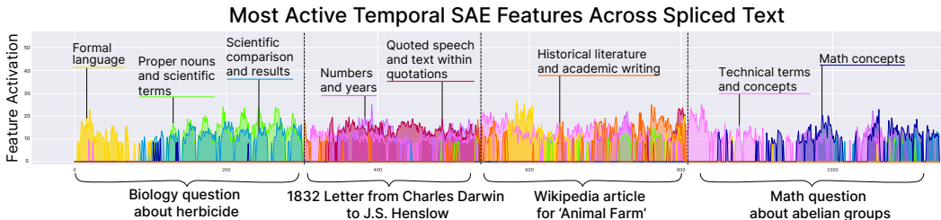
Figure 4: Top 8 most active Gemma2-2b Temporal SAE features over a concatenated sequence of text. Temporal SAE features exhibit clear phase transitions between sequences, are relatively smooth, and have explanations relevant to the semantic content of each component sequence.
