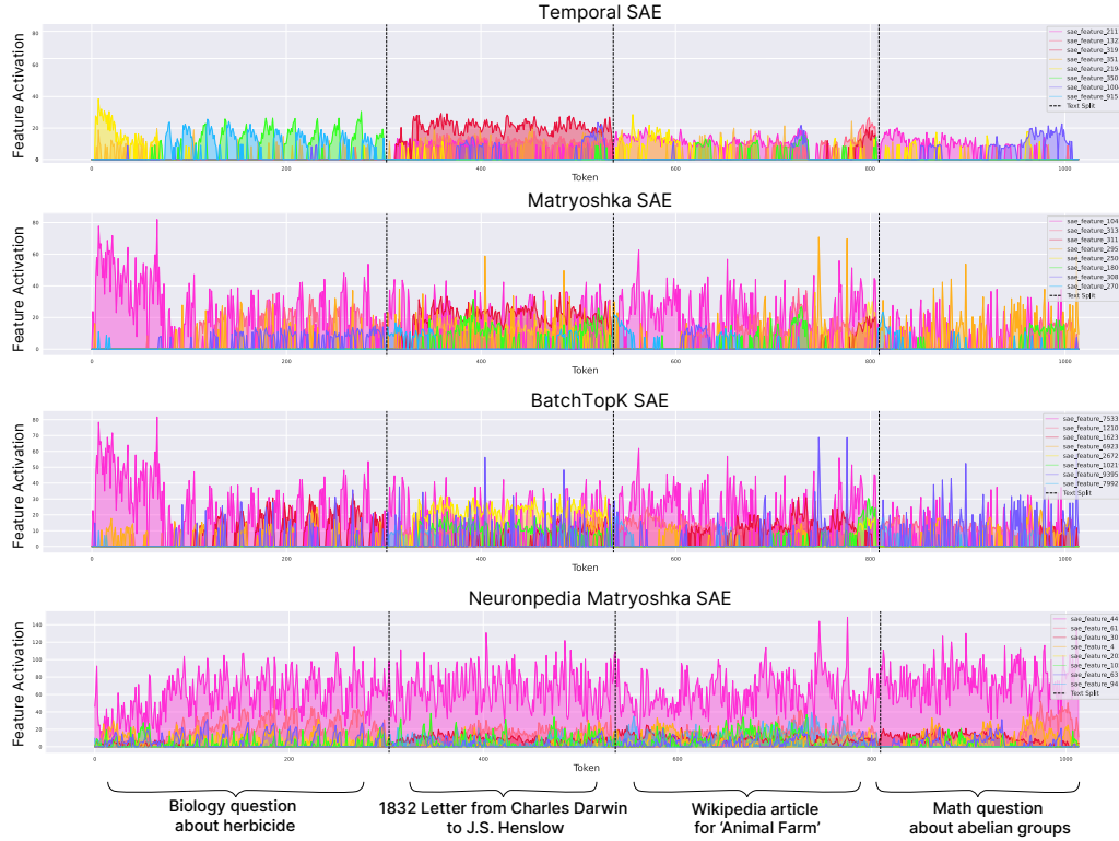
Figure 8: Top 8 most active features over the concatenated sequence of text used in Figure 4 for T-SAEs and baselines. Temporal SAE features exhibit clear phase transitions between sequences, are relatively smooth, and have explanations relevant to the semantic content of each component sequence. Baseline SAE features are much noisier or activate consistently over the entire sequence, without exhibiting separation between sequences.
