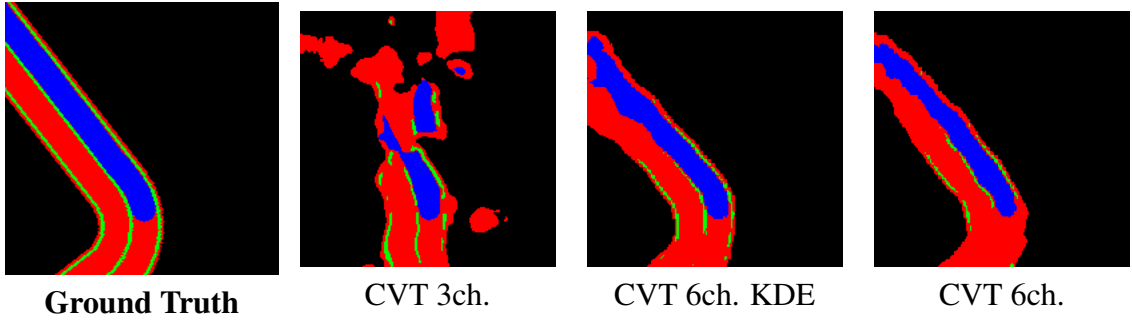
Figure 2. BEV predictions at the northwest curve of Town01 near the start of episode three, where the road transitions from an east–west straight to a southward turn. predictions at the same timestep. Only the CVT 6ch. and CVT 6ch. KDE agents complete this curve.
