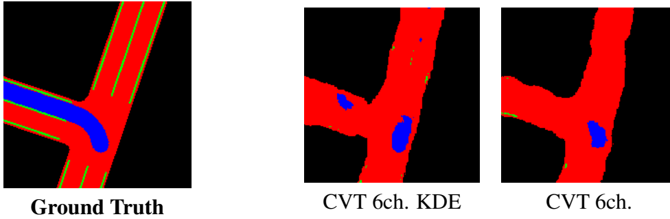
Figure 4. BEV predictions at the cross road in the east of Town02 when CVT 6ch. KDE and CVT 6ch. fail to make a left turn. Predictions at the same timestep.
