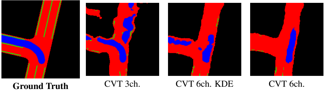
Figure 3. BEV predictions at the cross road in the middle of Town02 near the finish point of episode one. predictions at the same timestep. All agents fail in this intersection.
