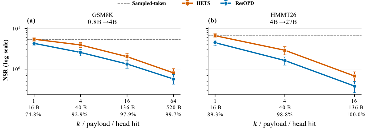
Figure 8: Comprehensive frozen-prefix support-size ( k ) diagnostics across benchmarks. ResOPD consistently reduces the dimensionless NSR across all evaluated support sizes on GSM8K and HMMT (log scale). Axis annotations detail the transmitted Teacher support size k , the corresponding communication payload (bytes/-token), and the empirical head-hit probability. Error bars denote 95% trajectory-level bootstrap confidence intervals.
