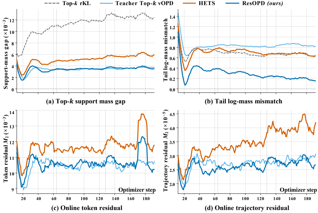
Figure 3: Training-time diagnostics (64 steps/epoch; lower is better). Panels (a) and (b) illustrate the student–teacher mismatch in Top- k support mass and tail log-mass across vOPD, HETS, ResOPD, and direct Teacher Top- k rKL. Panels (c) and (d) compare vOPD, HETS and ResOPD via the squared residual between the binary Top- k indicator and its student-predicted probability, evaluated at the token level and trajectory level, respectively. Detailed formulations are provided in Appendix D.1.
