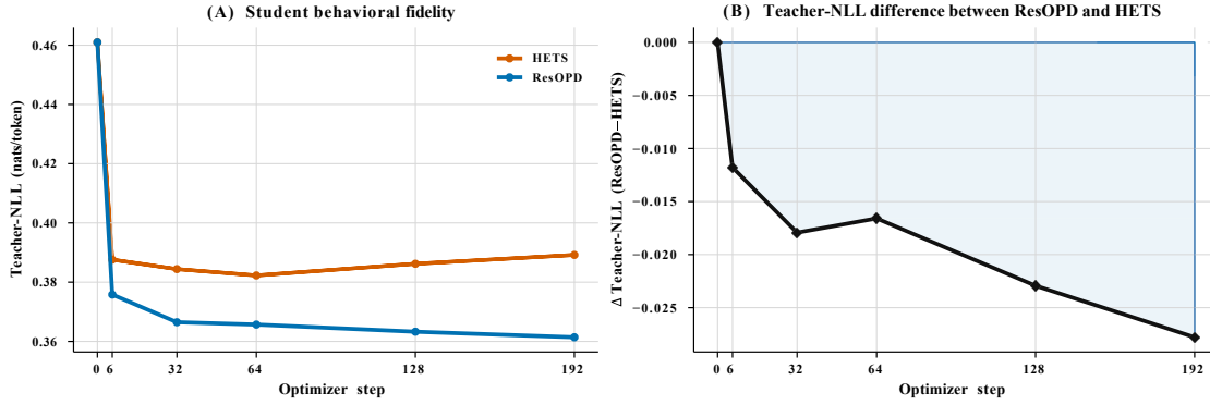
Figure 4: Teacher negative log-likelihood (NLL) across training in the Math OPD setup. Evaluations are computed over the four core benchmark families with identical weights to the main suite: AIME26, HMMT26, DeepMath held-out, and OlymMATH. Lower values indicate higher fidelity to the Teacher distribution.
