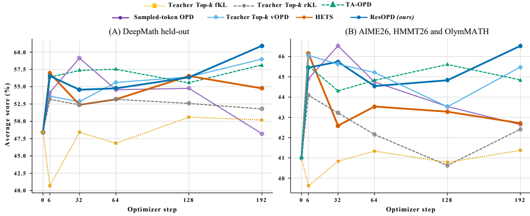
Figure 6: Step-wise learning curves corresponding to Tab. 3 on DeepMath held-out (left) and external competitions (right) across 192 optimizer steps.
