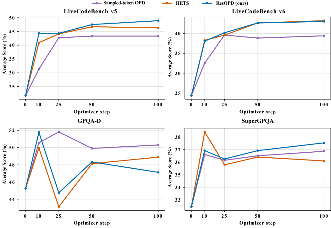
Figure 7: Evaluation trajectories during cross-domain transfer distillation from Qwen3-30B-A3B-Instruct to Qwen3-4B across optimizer steps (0, 10, 25, 50, and 100).
