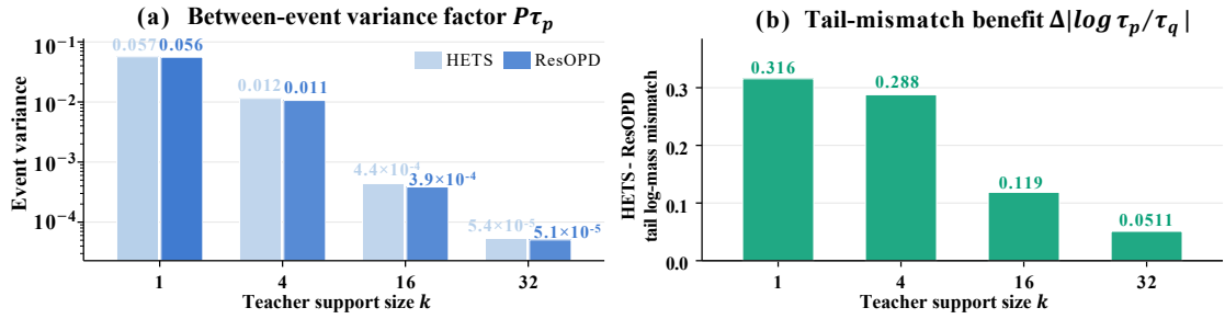
Figure 5: Online diagnostic metrics across teacher Top- k support sizes. (a) Between-event variance factor P_{\tau_p} for HETS and ResOPD, characterizing the scaling coefficient of the head-versus-tail partition. (b) Tail log-mass mismatch reduction (HETS – ResOPD, measured via \Delta |\log(\tau_p/\tau_q)| ).
