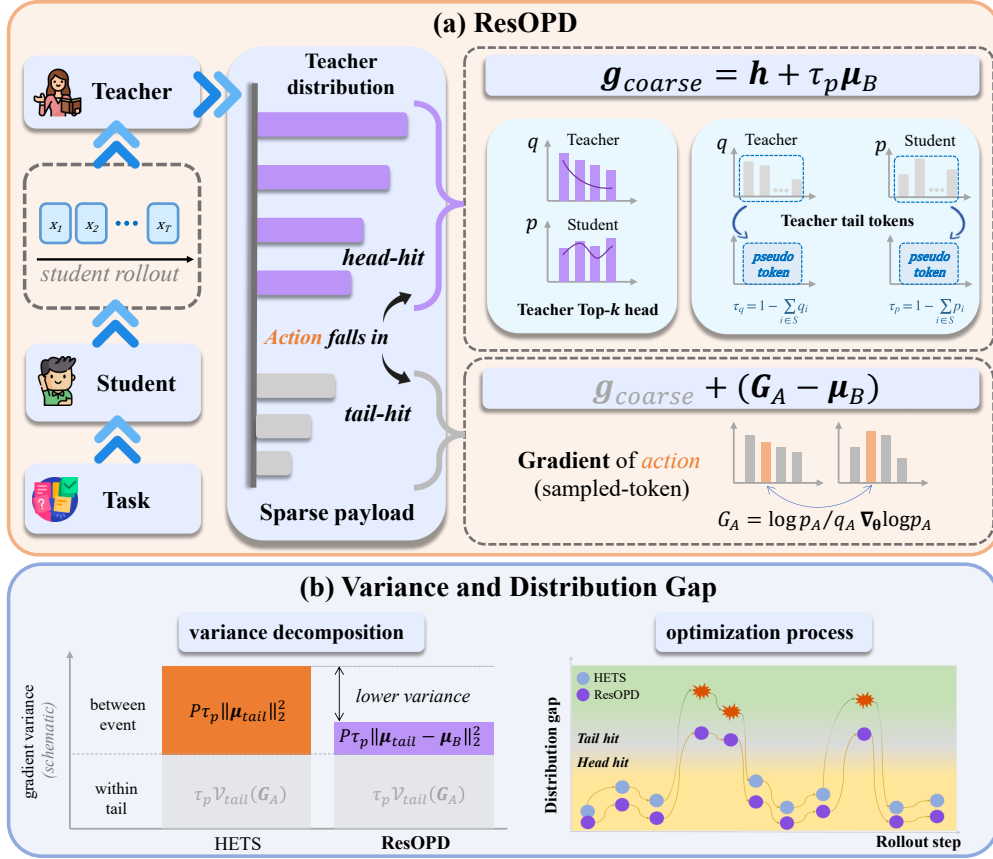
Figure 2: Overview of ResOPD. (a) When the student sampled-token falls in the head, ResOPD uses only the exact coarse gradient; upon a tail hit, it adds a residual correction. (b) ResOPD suppresses between-event variance compared to HETS by centering tail samples around \mu_B , achieving superior alignment with the teacher distribution across rollout steps.
