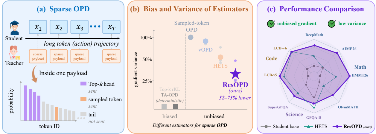
Figure 1: (a) Sparse OPD: the teacher model only sends the Top- k head probabilities and the sampled token score, leaving the tail distribution unobserved. (b) Bias vs. variance trade-off: while deterministic Top- k surrogates suffer from systematic gradient bias, ResOPD provides an unbiased gradient estimator and substantially reduces gradient variance. (c) Downstream evaluation: the radar chart shows benchmark scores across mathematics, coding, and science; while the relative ranking varies by task, ResOPD achieves the best overall performance.
