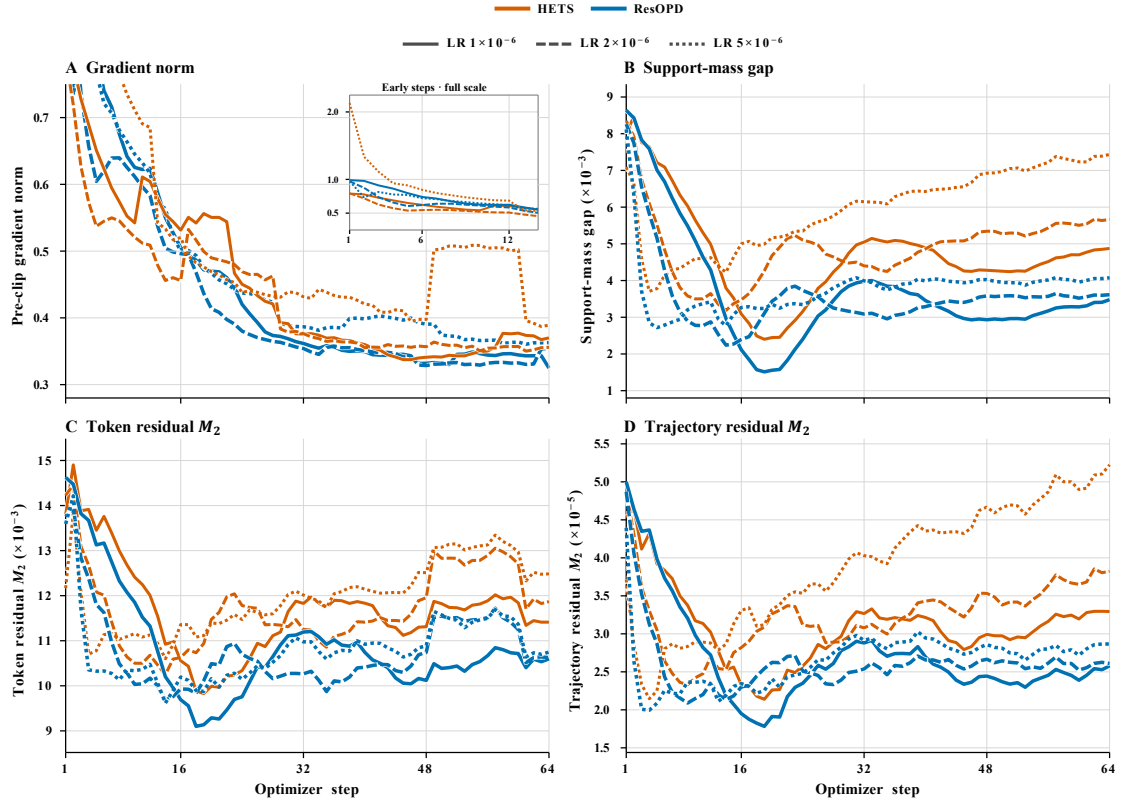
Figure 9: Training dynamics and learning-rate sensitivity of HETS (orange) vs. ResOPD (blue) on DeepMath across three learning rates ( 1 \times 10^{-6} solid, 2 \times 10^{-6} dashed, 5 \times 10^{-6} dotted). (A) Pre-clipping global gradient norm (inset displays full-scale unclipped peaks over early steps). (B) Support-mass gap ( Q - P ) on the transmitted Teacher Top-4 tokens. (C, D) Token-level and trajectory-level second residual moments ( M_2 ). While HETS exhibits large gradient-norm excursions and growing mass/residual discrepancies as the learning rate scales up to 5 \times 10^{-6} , ResOPD maintains stable dynamics and stays close to its low-rate trajectories throughout optimization.
