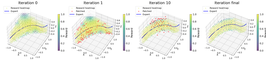
Fig. 2. 3D spatial Flywheel progression. The learned Oracle initially assigns non-trivial reward to many cells outside the expert-path basin. Governance batches add suppression kernels around verified flaw regions. Across iterations, the active reward surface contracts toward the expert trajectory while the sampled basin is preserved.
