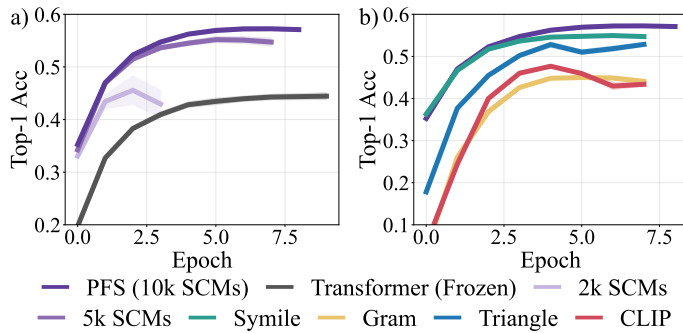
Figure 3: Validation performance of well-tuned baselines, the frozen Transformer and the PFS on the UKB. a) Scaling the prior-fitting with more sampled SCMs improves transfer to real-world data. b) Using the frozen PFS leads to faster convergence and higher retrieval accuracy than the baselines.
