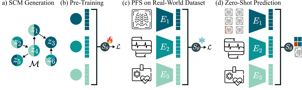
Figure 1: Overview of the Prior-Fitted Scorer (PFS), illustrated on the trimodal MIMIC-Symile setting (Saporta et al., 2024). (a) We sample latent causal structures and generate synthetic multimodal tuples from an SCM prior \mathcal{M} . (b) A Transformer scoring function s_\theta is pretrained on these synthetic tuples to distinguish compatible from mismatched multimodal combinations with loss \mathcal{L} , thereby shaping its inductive bias. (c) The PFS is transferred to the real dataset and kept frozen while the modality encoders E_i are optimized through the contrastive objective. (d) After extensive tuning, the PFS is evaluated on zero-shot predicting the future chest X-ray. Overall, a PFS replaces a manually specified similarity function with a Transformer whose structure is learned from a synthetic causal prior.
