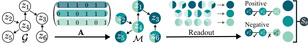
Figure 2: Overview of synthetic multimodal data generation and contrastive prior-fitting. A DAG \mathcal{G} defines causal dependencies among latent variables, while the binary assignment matrix \mathbf{A} selects the latent subsets contributing to each modality, inducing shared, subset-specific, and modality-private information. The selected latent variables are combined through linear and nonlinear readouts to produce modality vectors. During prior-fitting, matched tuples contain modalities from the same synthetic sample, whereas negatives are formed by replacing the target modality with a sampled mismatched candidate before scoring with s_\theta .
