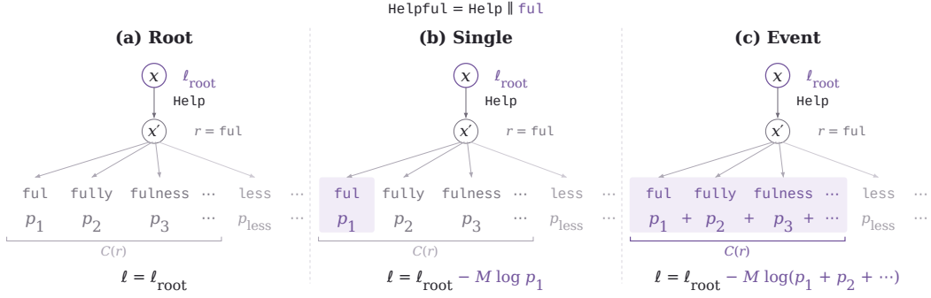
Figure 6: One-step completion and supervision choices. Sampling Help leaves residual r = \text{ful} for the representative event Helpful. Valid one-token completions include ful, fully, and fulness; less lies outside \mathcal{C}(r) . All three objectives share the same root loss and student predictions. (a) Root adds no child loss. (b) Single supervises one selected completion. (c) Event supervises the completion set’s total probability. Here, p_i denotes a candidate’s native student probability at x' , and M is the representative group’s teacher mass. Ellipses indicate additional candidates. Tokenizations and the Single selection are illustrative; losses are shown for one group before training-mask reduction.
