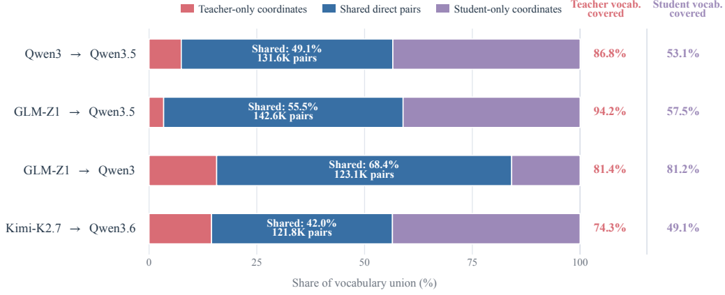
Figure 5: Static Teacher-Student vocabulary overlap. Bars show Teacher-only, shared, and Student-only shares of the vocabulary union; right-hand columns report directional coverage.
