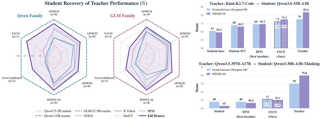
Figure 1: Cross-tokenizer distillation results across model scales. Left: Teacher-normalized pass@ n scores on six mathematics and code benchmarks, with Qwen3.5-2B distilled from Qwen3-32B or GLM-ZI-9B. Recovery is the Student score divided by the corresponding teacher score, expressed as a percentage; 100% indicates matching teacher performance. We use n = 8 for mathematics and n = 2 for code. Right: Absolute scores on FrontierScience Olympiad and PHYRD-40 for two large-scale heterogeneous MoE pairs. Together, these results show consistent improvements across task domains, model families, and scales.
