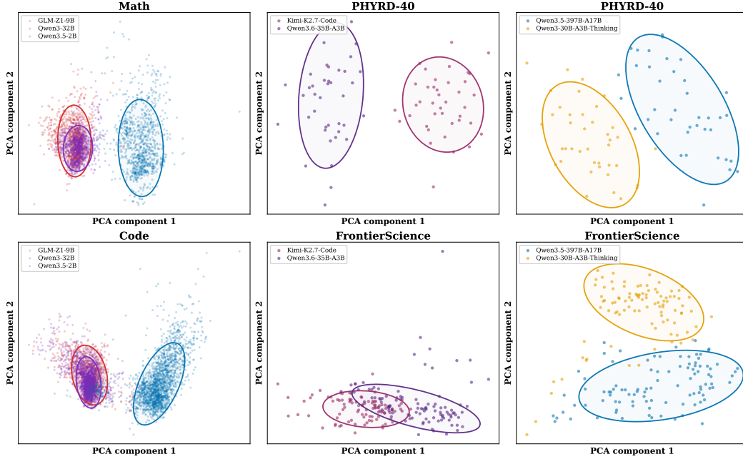
Figure 7: PCA projections of response-level reasoning features across math, code, and scientific reasoning benchmarks. Each point represents a generated response, with colors identifying models; ellipses summarize response distributions after robust trimming. PCA is fitted separately in each panel, so distances and directions are comparable only within panels.
