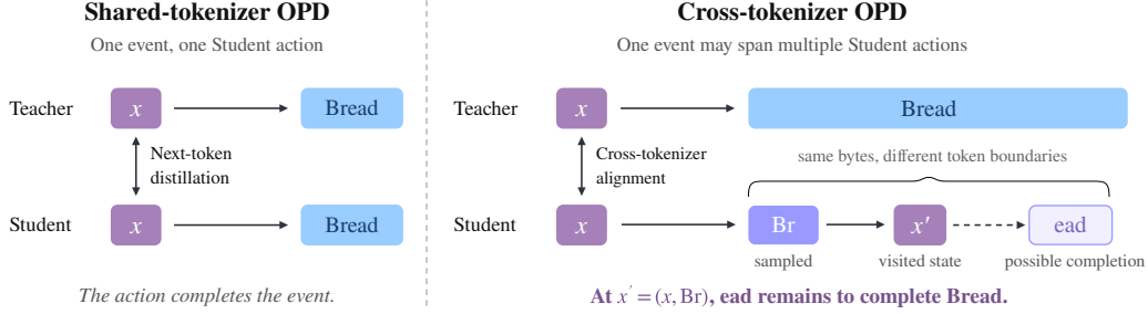
Figure 2: On-policy distillation with shared and different tokenizers. Left: a shared tokenizer allows direct next-token supervision. Right: a teacher token such as Bread may span multiple student actions. After sampling Br , the student reaches x' = (x, \text{Br}) with residual bytes ead still required to complete the event. The dashed arrow indicates a possible continuation, highlighting the distinction between entering an event and completing it.
