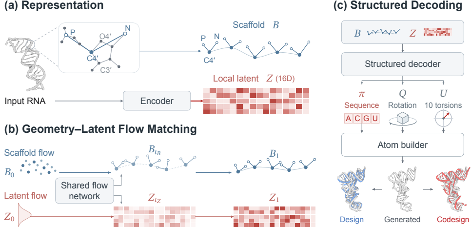
Figure 1: Overview of La-Ribo. (a) Each residue is represented by an explicit P/C4'/glycosidic-N scaffold (blue) and an encoded 16-dimensional latent (red). (b) A shared flow network jointly generates states with modality-specific schedules. (c) The frozen decoder predicts nucleotide identity, a scaffold-to-sugar rotation, and torsions, from which the atom builder builds all heavy atoms.
