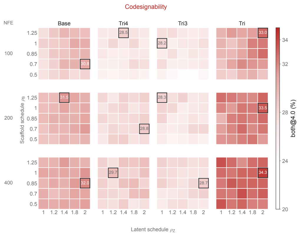
Figure 11: Strict codesignability on the schedule grid of Figure 10. Panels share a color scale, and black outlines mark maxima.
