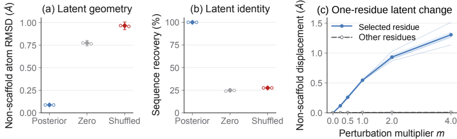
Figure 2: Latent interventions with a fixed scaffold. (a,b) compare posterior-mean, zero, and shuffled latents; (c) shows atom displacement from a separate one-residue latent perturbation.
