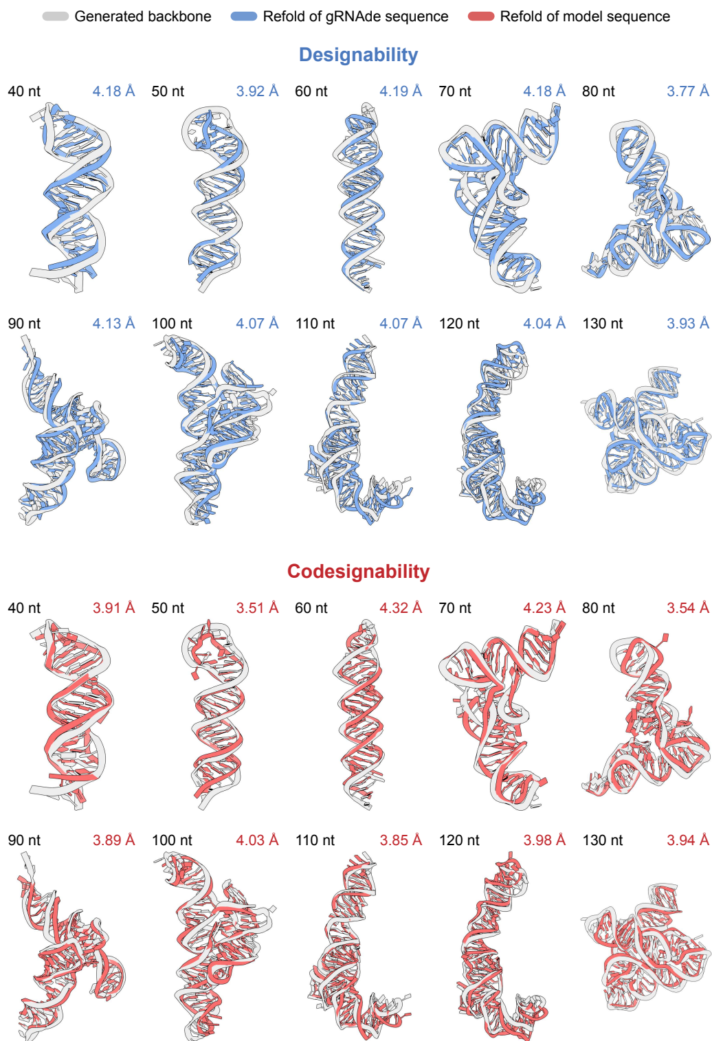
Figure 6: La-Ribo backbones (40–130 nt, grey) overlaid with refolds of the best of eight gRNAd sequences (top) and the co-designed sequence (bottom). Numbers: C4' scRMSD (Å).
