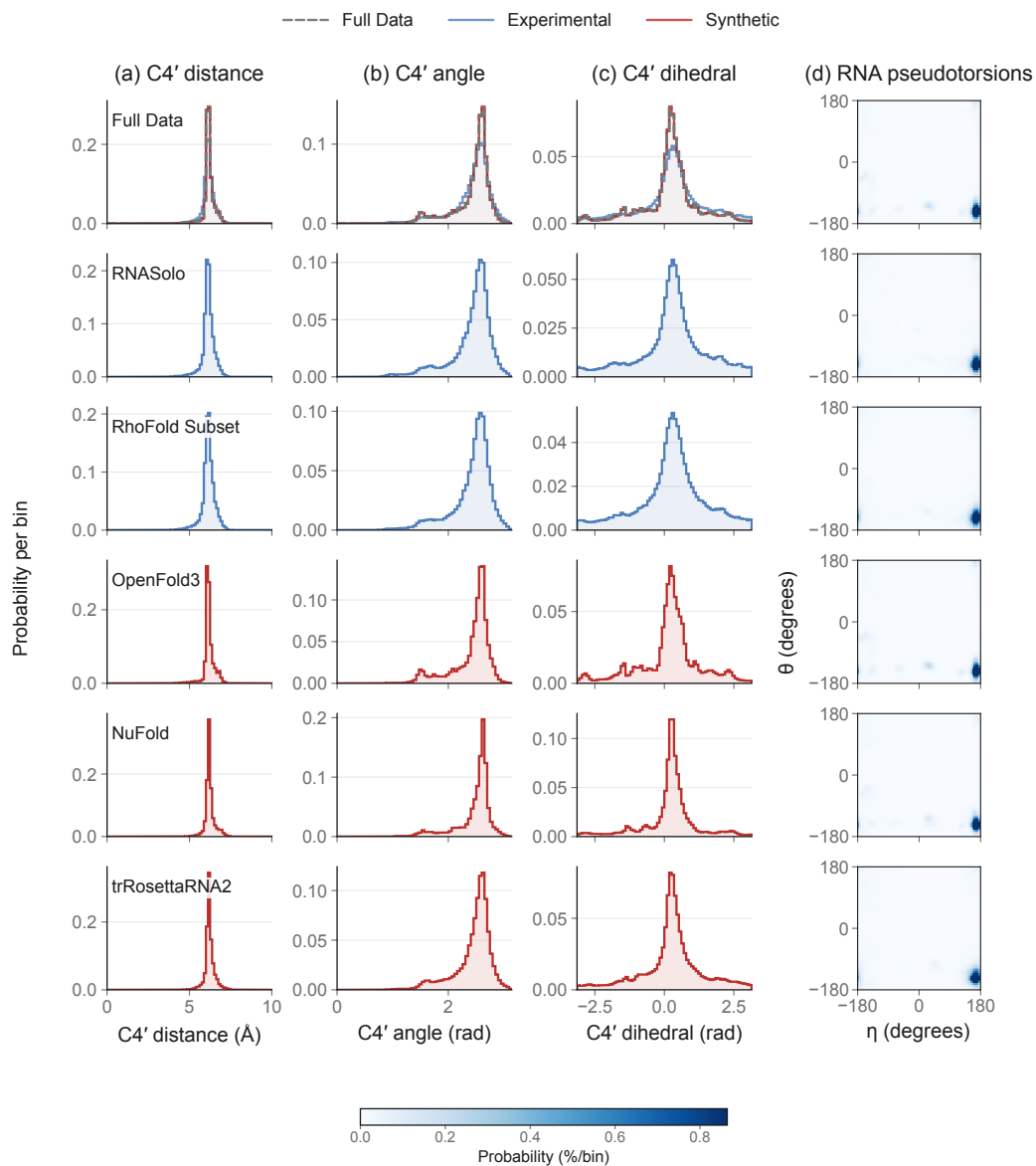
Figure 7: Local geometry by corpus source. Rows show the pooled corpus and individual sources; columns show C4' distance, angle, dihedral, and joint ( \eta, \theta ) density. In the pooled row, blue and red outlines distinguish experimental and synthetic structures. Histograms are normalized within each cohort; density panels share a color scale.
