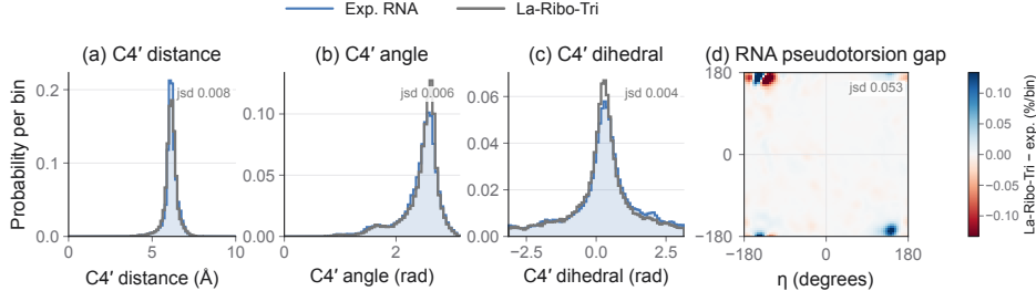
Figure 4: Local geometry of La-Ribo-Tri (gray) and experimental RNA (blue; RNASolo and RhoFold PDB). (a–c) compare C4' distance, angle, and dihedral; (d) shows generated-minus-experimental pseudotorsion density. JSD is in bits.
