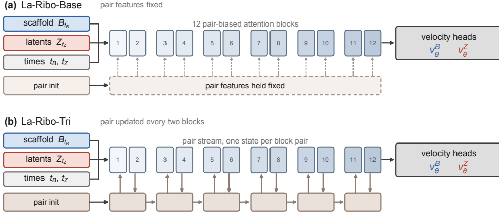
Figure 9: Base and Tri flow architectures. Both use a 12-block trunk to predict scaffold and latent velocities. La-Ribo-Base keeps pair features fixed as attention biases; La-Ribo-Tri updates them every two blocks using token-to-pair projections and triangle multiplicative updates.
