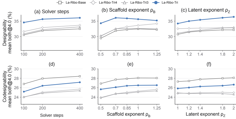
Figure 5: Sampling sensitivity. Columns show solver steps, scaffold power \rho_B , and latent power \rho_Z ; top/bottom rows show marginal strict both@4.0 designability/codesignability.
