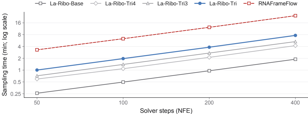
Figure 12: Generation time for 600 RNAs by solver steps, excluding inverse folding, refolding, and scoring. La-Ribo uses eight A800 GPUs; RNA-FrameFlow time is throughput-normalized. Timing scopes differ; steps are categorical and time is logarithmic.
