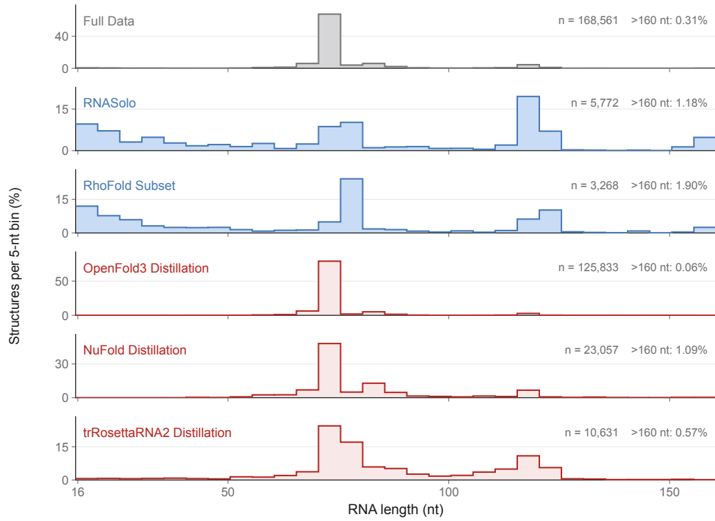
Figure 8: Length distributions of 168,561 eligible RNAs, pooled (top) and by source. Histograms are row-normalized; labels report the fraction above 160 nt. Gray, blue, and red denote pooled, experimental, and synthetic structures.
