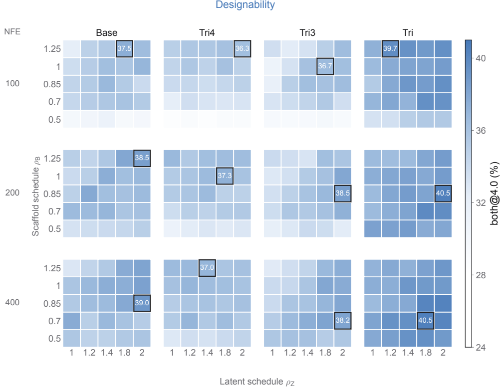
Figure 10: Strict designability across modality schedules and four architectures. Rows show 100, 200, and 400 steps; each schedule-pair cell contains 600 RNAs. Panels share a color scale, and black outlines mark maxima.
