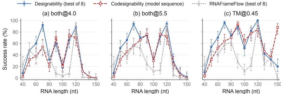
Figure 3: Length-resolved La-Ribo-Tri success at 200 steps for one 600-RNA campaign (50 RNAs per length). Error bars show 95% Wilson intervals.
