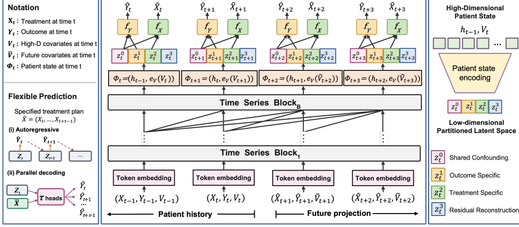
Figure 1: Overview of HiSTOR. The model adopts a temporal Transformer backbone and combines a high-dimensional current patient state with a learned representation of longitudinal history, maps their fusion into a structured latent space, and supports treatment-conditioned flexible one-step and multi-step outcome prediction.
