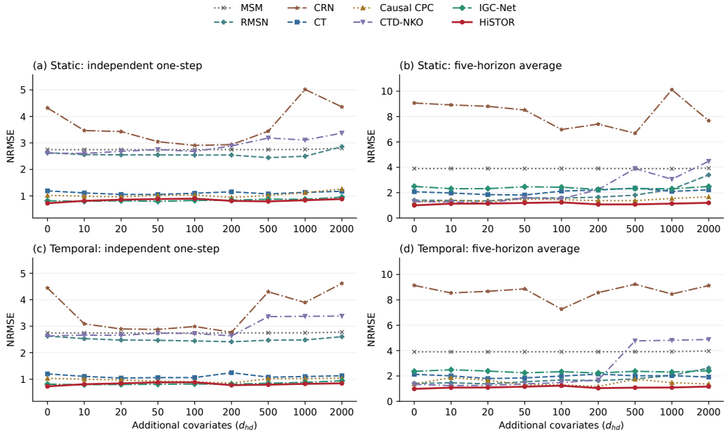
Figure 4: All eight methods across the complete CVSim dimension grid. Lines show five-seed mean NRMSE.
