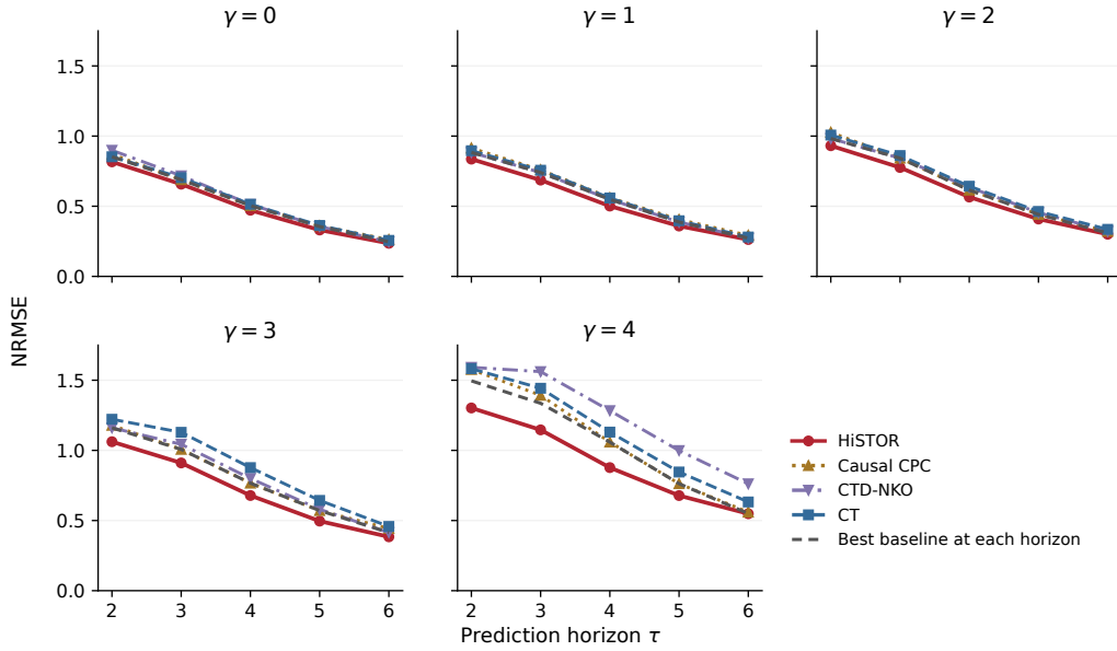
Figure 2: CancerSim sustained-treatment NRMSE over \tau = 2, \dots, 6 . Lines are five-seed means; the gray envelope is the lowest mean among all baselines at each horizon and may switch methods. Complete results and SDs are in Appendix G.
