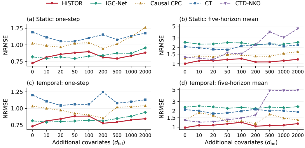
Figure 3: CVSim NRMSE across nine d_{hd} settings. Panels (a,b) show Static and panels (c,d) Temporal results; the left panels report independent one-step error and the right panels report five-horizon means. Lines are five-seed means. Appendix Figure 4 includes all methods.
