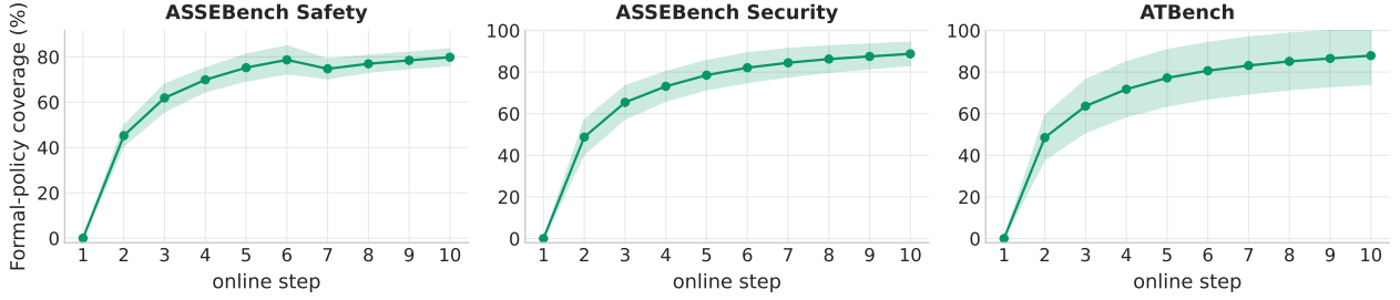
Figure 4 | Growth of active formal-policy coverage across deployment rounds, measuring the fraction of unseen events for which VEPA makes a symbolic allow-or-refuse decision.
