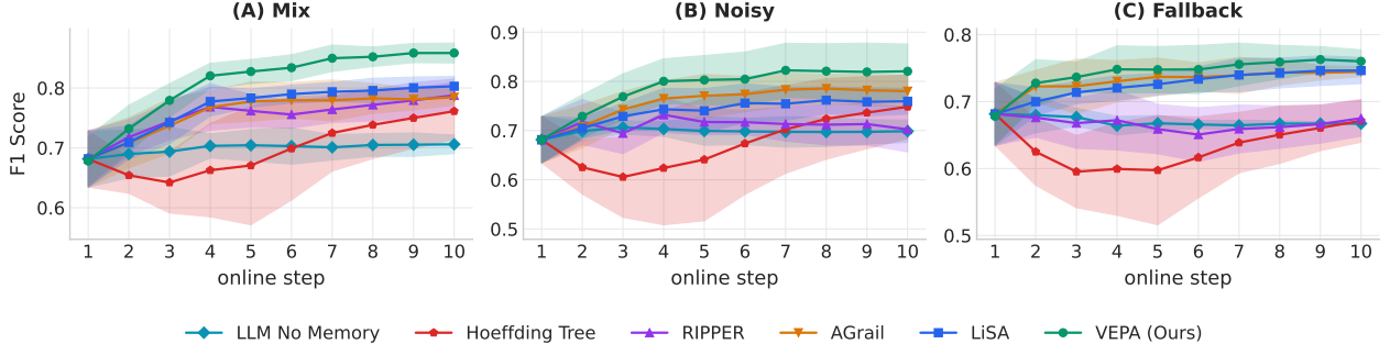
Figure 5 | Performance under realistic deployment conditions. (A) Mixed-stream evaluation combining three benchmarks, testing adaptation across heterogeneous and shifting risk types. (B) Robustness to noisy feedback, where revealed adaptation labels are independently corrupted before each update. (C) Full-stream hybrid deployment, where events covered by the active formal policy receive its deterministic decision and uncovered events are routed to the deployment-time LLM fallback.
