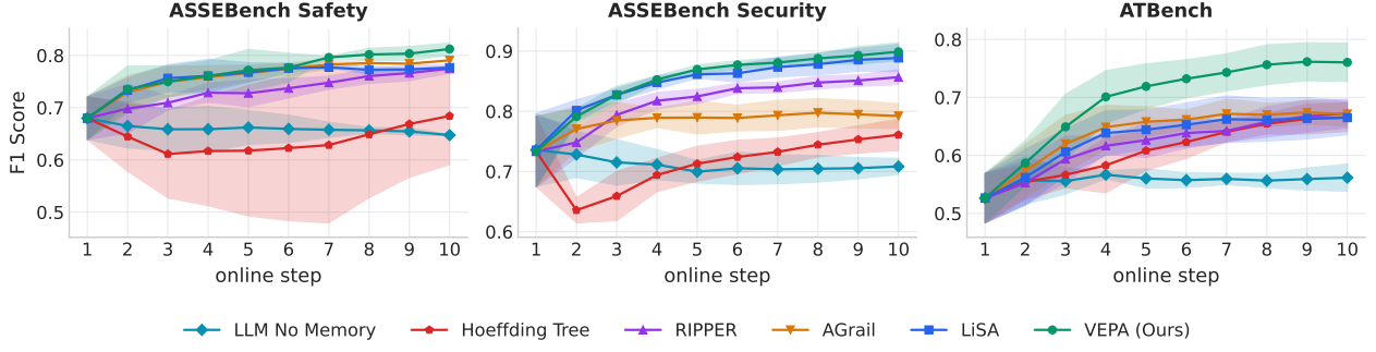
Figure 3 | Decision quality on events covered by the active formal policy, with all baselines evaluated on the same examples before each deployment update.
