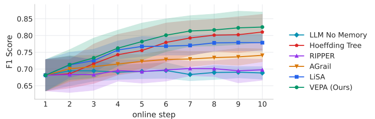
Figure 10 | Performance under targeted adversarial feedback on the mixed deployment stream. Corrupted feedback is concentrated on prompt-injection examples.
