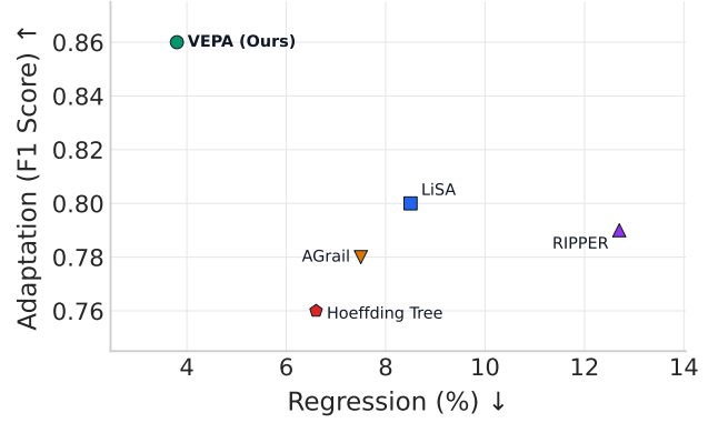
Figure 11 | Adaptation-regression trade-off across methods on the mixed deployment stream.
