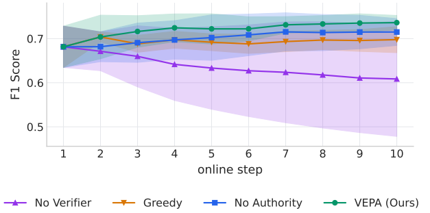
Figure 6 | Ablation study of VEPA on the mixed deployment stream experiment
