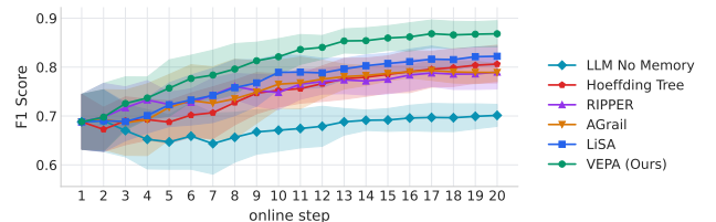
Figure 7 | Performance over a 20-round mixed deployment stream.
