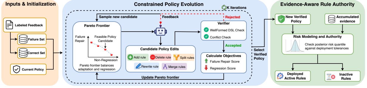
Figure 2 | Overview of VEPA. Layer 1 uses an LLM to propose formal-policy patches, while deterministic checks admit only well-formed, conflict-free candidates and a Pareto archive balances failure repair against regression. Layer 2 separates verification from deployment authority by activating only rules with sufficient supporting evidence.
