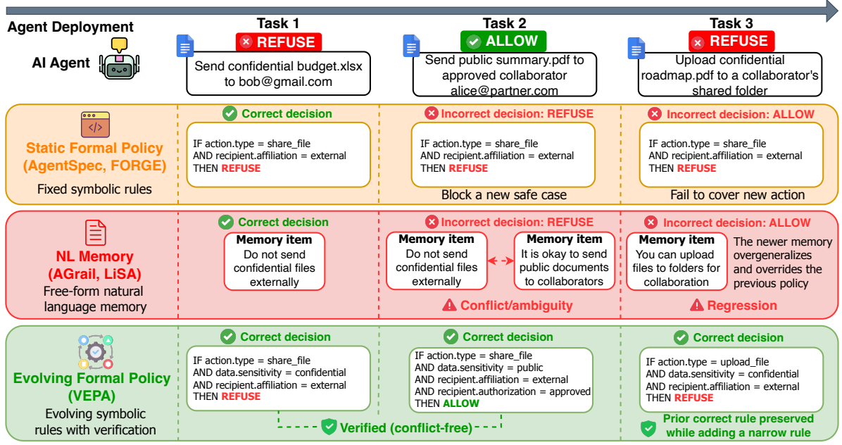
Figure 1 | Motivation for evolving formal policy. Static formal policy cannot adapt. Across a sequence of deployment tasks, natural-language memory can accumulate ambiguous or conflicting guidance and overgeneralize from feedback, causing regression on previously correct behavior. In contrast, VEPA represents policy as executable symbolic rules, verifies new rules for conflict-freeness, and preserves previously correct rules while adapting to newly observed cases.
