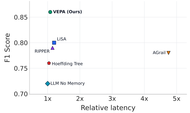
Figure 14 | F1 versus relative inference latency. Latency is reported relative to the deployment-time reference used in the experiment.
