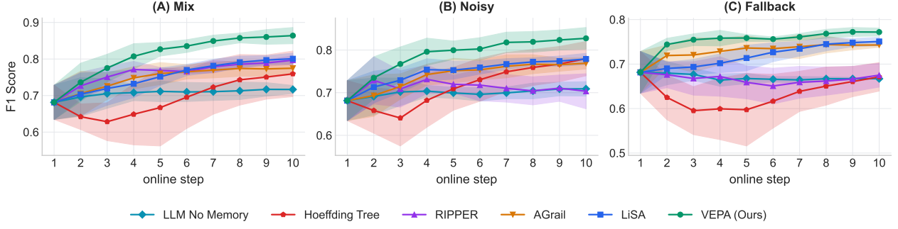
Figure 8 | Mixed-stream performance when replacing the update-time policy proposer with Gemini-3.6-Flash.
