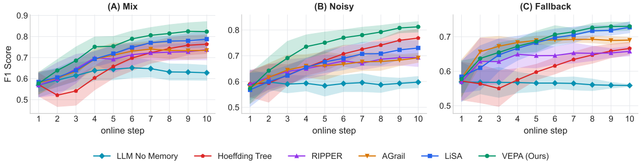
Figure 9 | Mixed-stream performance when replacing the deployment-time parser and inference model with Gemini-3.5-Flash-Lite.
