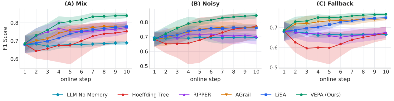
Figure 13 | Performance of different methods using Qwen-3.8-27B.
