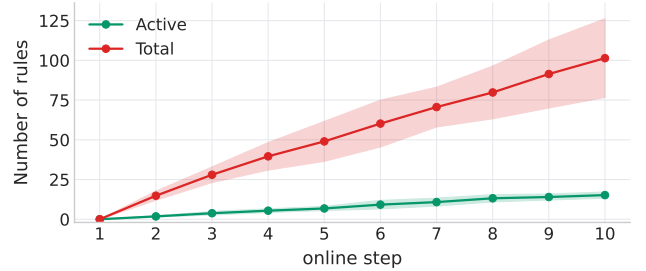
Figure 12 | Growth of the verified rule archive and the subset of rules granted active authority.
