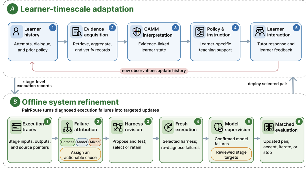
Figure 2: RegulaTutor adapts at two timescales. During tutoring, accumulated learner history supports evidence acquisition, CAMM-guided interpretation, and learner-specific instructional policies that update with new interactions. Offline, PairRoute attributes execution failures to the harness, model, or both and routes them to targeted harness revision or reviewed model supervision. The updated model–harness pair is evaluated before the next round or deployment.
