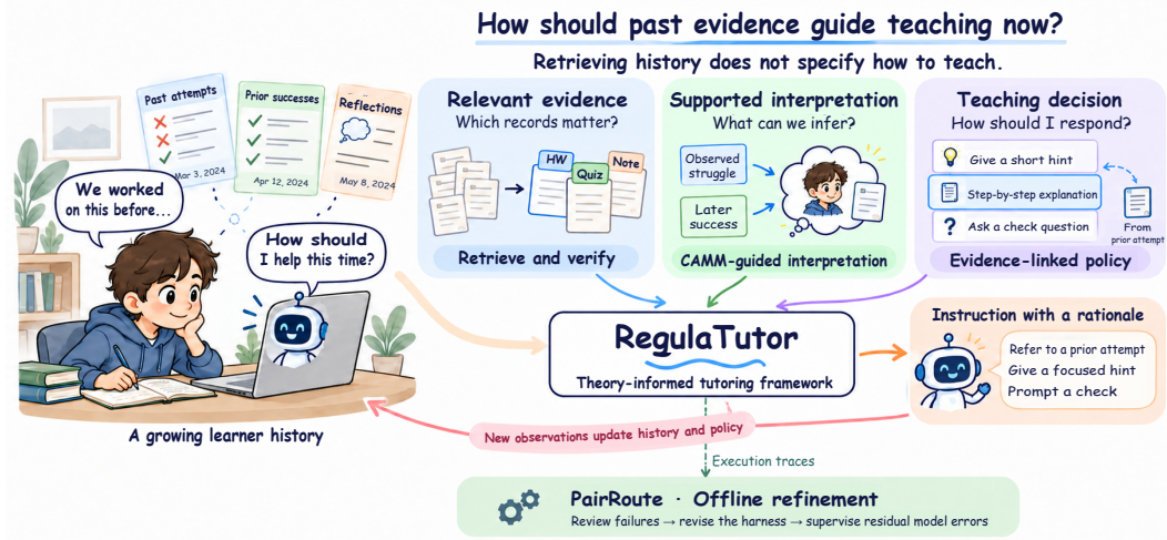
Figure 1: RegulaTutor connecting learner history to instructional decisions. The learner–tutor setting (left) motivates three questions (top): which records are relevant, what interpretations they support, and how those interpretations should guide teaching. RegulaTutor makes these connections explicit through CAMM-guided learner interpretation and evidence-linked teaching policies, with learner history and policies updated as new observations arrive. PairRoute (bottom) uses execution traces to guide offline harness revisions and construct reviewed stage-level supervision for residual model errors.
