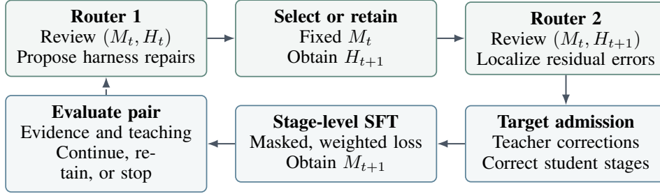
Figure 3: A PairRoute round. Harness selection precedes the construction of model supervision. Trajectories may be reused when the selected model–harness pair is unchanged.
