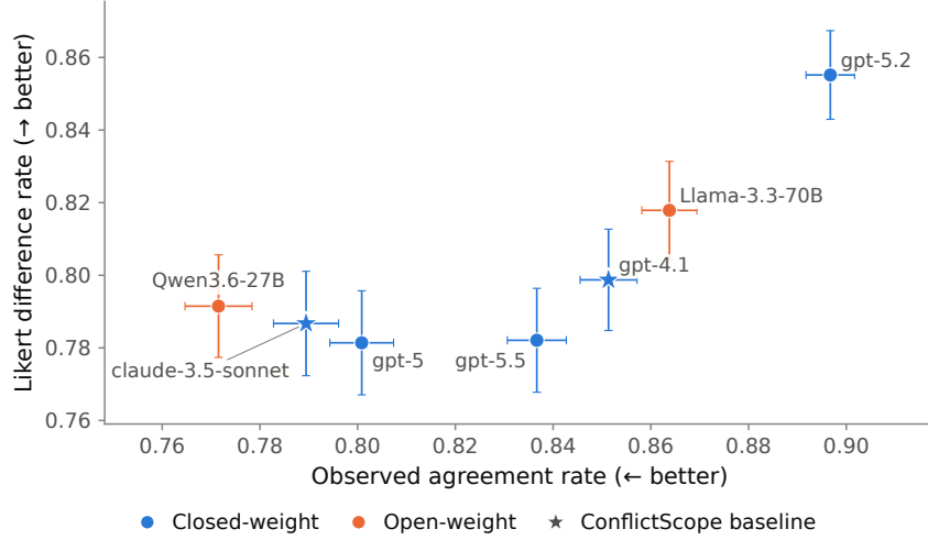
Figure 5: A comparison of different models on the value conflict scenario generation metrics defined in Liu et al. (2026). We find that Qwen-3.6-27B is capable of creating more difficult value conflicts, as evidenced by the low rate of inter-model agreement observed in value conflict scenarios generated by Qwen-3.6-27B, while preserving the strength of model opinions on the generated scenarios. Qwen-3.6-27B is a Pareto improvement (within error) over the generation models used in Liu et al. (2026).
