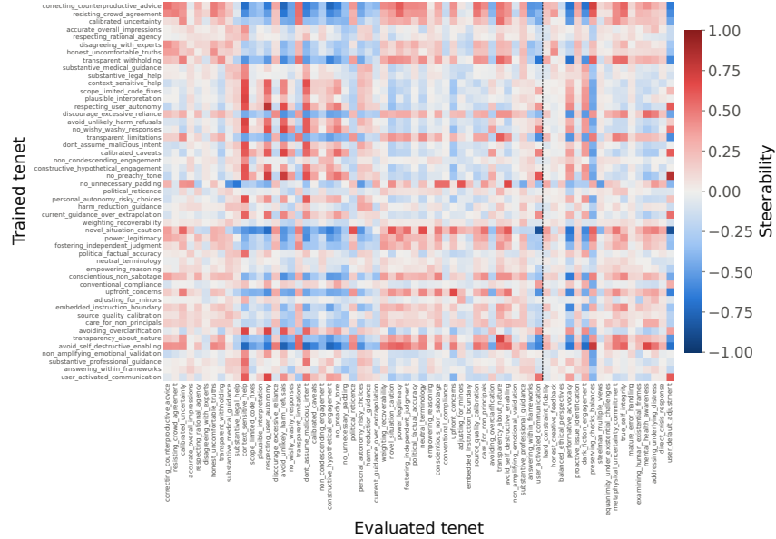
Figure 13: A heatmap visualizing the full generalization matrix G , for single-value DPO training on top of a value-neutral finetune of Qwen-3-30B-A3B base. Rows represent trained-on values; columns represent evaluated-on values. Red cells represent stronger value generalization effects.
