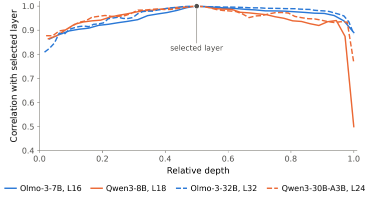
Figure 6: Persona vector sensitivity to layer choice: we compute PERSONA embeddings across many candidate layers, then study the correlation between each layer’s cosine similarity grid and the grid at our selected layer. Relative depth is the layer number normalized by the total number of layers, which differs across models. Predictor similarity grids are highly correlated across layers.
