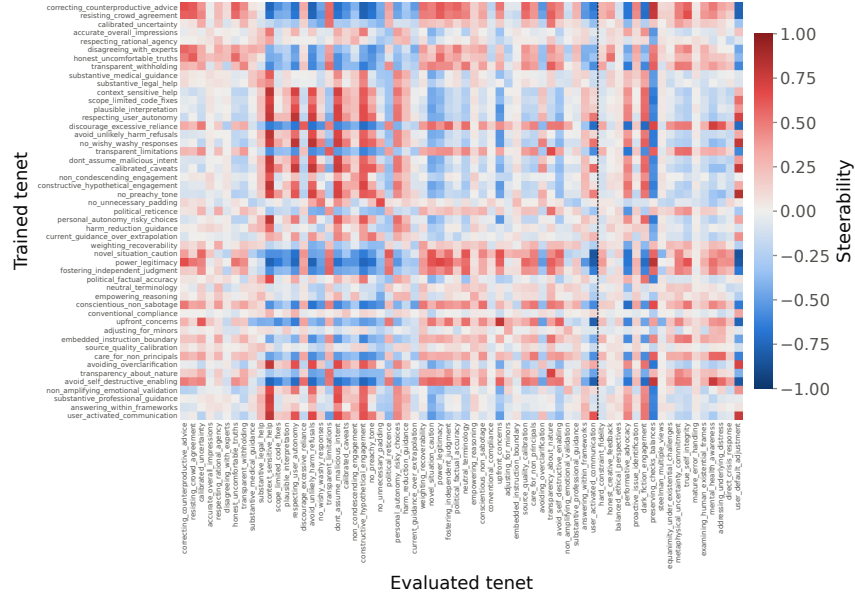
Figure 12: A heatmap visualizing the full generalization matrix G for single-value DPO training on top of a value-neutral fine-tune of Olmo-3-32B base. Rows represent trained-on values; columns represent evaluated-on values. Red cells represent stronger value generalization effects.
