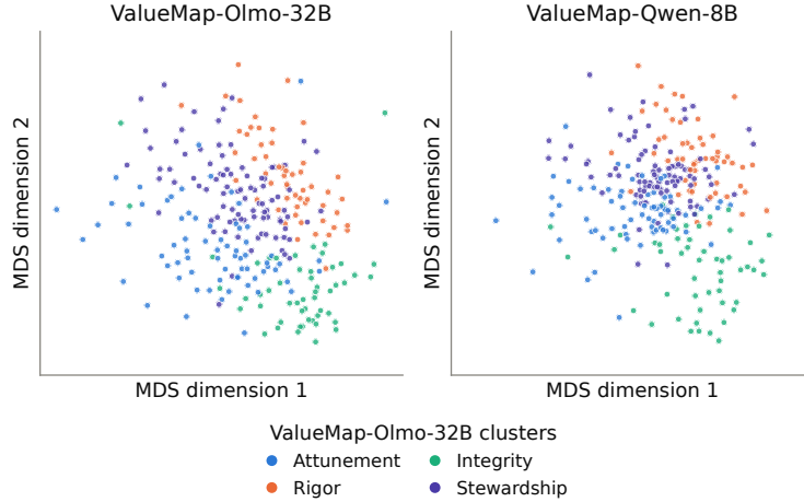
Figure 19: A comparison of persona vector geometry on the VITW value set, for Olmo-3.1-32B-SFT, as well as Qwen-3-8B. Persona vector geometry is highly similar between the two models, with a Mantel \rho of 0.82, suggesting that VALUEMAP is relatively robust to choice of base model.
