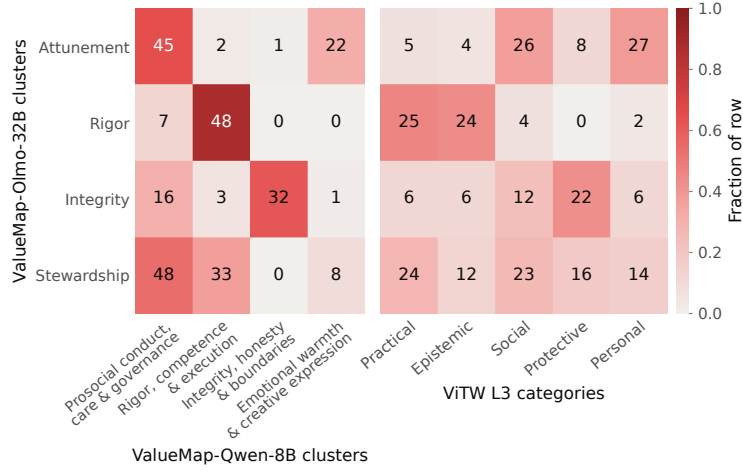
Figure 20: A comparison of cluster assignments for each of the 266 VITW values, between two variants of VALUEMAP computed on different models, as well as between VALUEMAP (Olmo 32B) and the original Values in the Wild categories. We find moderate similarity between VALUEMAP variants between different models, and lower similarity between VALUEMAP and Values in the Wild.
