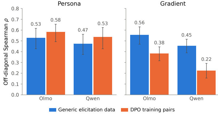
Figure 17: A comparison of value representation quality across different elicitation datasets, for the DPO interventions. We find that using actual DPO training pairs as elicitation data only leads to modest improvements in PERSONA representation quality, and a sharp decrease in GRADIENT representation quality, as measured in Spearman \rho on a 49 \times 49 subset of the matched generalization matrix.
