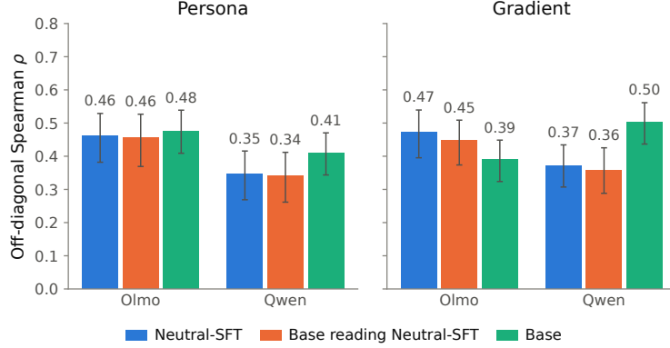
Figure 16: A comparison of value representation quality across different elicitation datasets, for SFT interventions at 7-8B scale. We find that using the base model with an instruction-following template leads to higher average correlation between representation similarity and ground-truth generalization matrices, compared to using a finetuned base with higher instruction-following capabilities.
