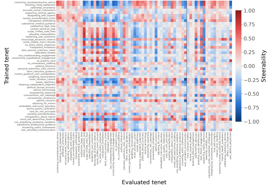
Figure 8: A heatmap visualizing the full generalization matrix G for single-value DPO training on top of a value-neutral fine-tune of Olmo-3-7B base. Rows represent trained-on values; columns represent evaluated-on values. Red cells represent stronger value generalization effects.
