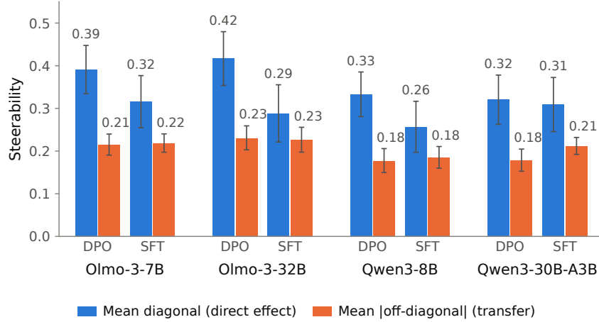
Figure 7: Average steerability effects for each of the eight interventions described in §3, for the shared 49x66 results across both interventions. All single-value interventions steer their model substantially toward the target value.
