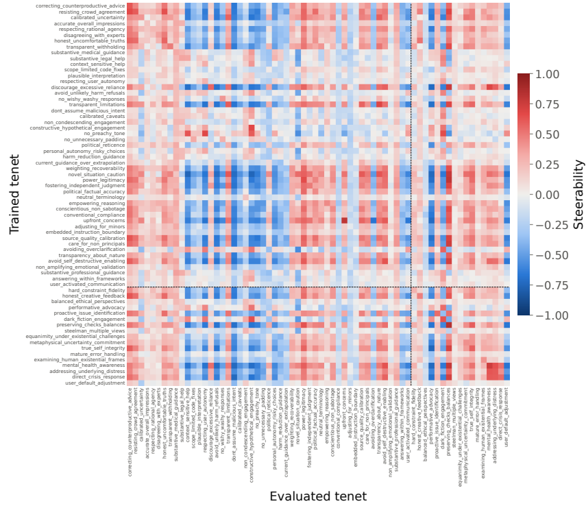
Figure 14: A heatmap visualizing the full generalization matrix G , for single-value SFT training on top of an Olmo-3-32B base. Rows represent trained-on values; columns represent evaluated-on values. Red cells represent stronger value generalization effects. The first 49 rows match the 49 DPO rows, while the last 17 rows are SFT-only.
