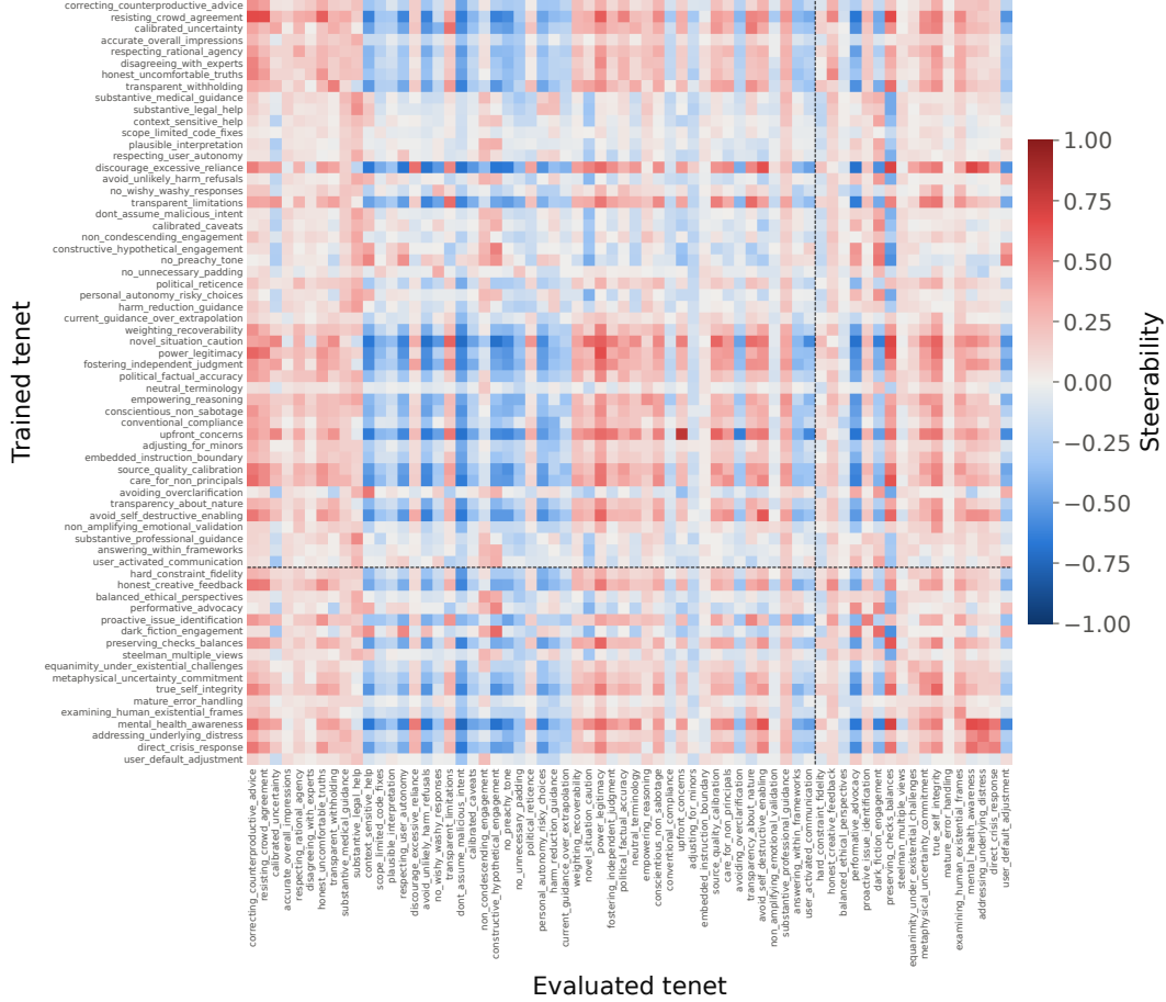
Figure 11: A heatmap visualizing the full generalization matrix G , for single-value SFT training on top of a Qwen-3-8B base. Rows represent trained-on values; columns represent evaluated-on values. Red cells represent stronger value generalization effects. The first 49 rows match the 49 DPO rows, while the last 17 rows are SFT-only.
