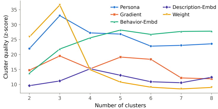
Figure 18: Adjusted silhouette scores for clusterings computed with k -medoids over the CONSTITUTION set, across a range of k values and value embedding methods. We find that PERSONA achieves the highest mean adjusted silhouette score, as well as the highest total adjusted silhouette score (excluding a degenerate clustering computed with WEIGHT at k = 3 ). This motivates the selection of the PERSONA - k -medoids combination to create VALUEMAP.
