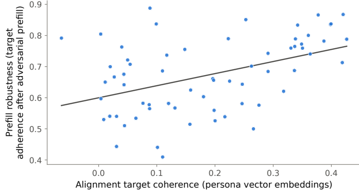
Figure 3: Coherence of the 64 alignment targets and their models’ adversarial robustness. We find a significant correlation between alignment target coherence and the prefill robustness of models trained on said alignment targets (Spearman \rho = 0.43 , p = 5 \times 10^{-4} ). This validates our hypothesis in §5 and shows the utility in applying PERSONA representations toward the study of multi-value training effects.
