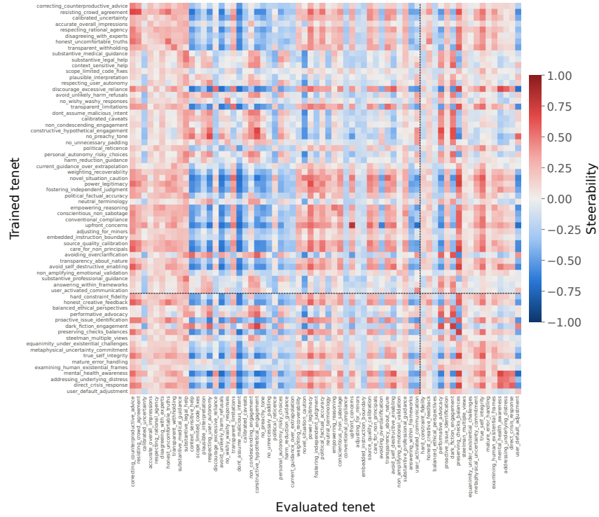
Figure 10: A heatmap visualizing the full generalization matrix G , for single-value SFT training on top of an Olmo-3-7B base. Rows represent trained-on values; columns represent evaluated-on values. Red cells represent stronger value generalization effects. The first 49 rows match the 49 DPO rows, while the last 17 rows are SFT-only.
