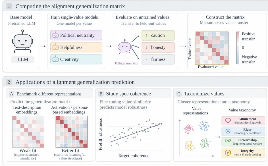
Figure 1: Overview of our contributions. We conduct a large-scale study of single-value generalization, i.e., how aligning a model to a single value influences its alignment toward other values. We introduce an alignment generalization prediction task, evaluating value representations by how well their pairwise similarity correlates with the ground-truth generalization matrix. Finally, we apply the most predictive representations to multi-value alignment target analysis and value taxonomization.
