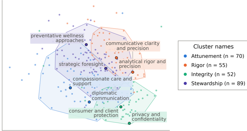
Figure 4: A visualization of how VALUEMAP classifies the set of 266 Values in the Wild values using Olmo-3.1-32B-SFT. MDS is used to project all value representations onto a 2D plot. Shaded regions represent the convex hull of the 90% of points in each category closest to its centroid.
