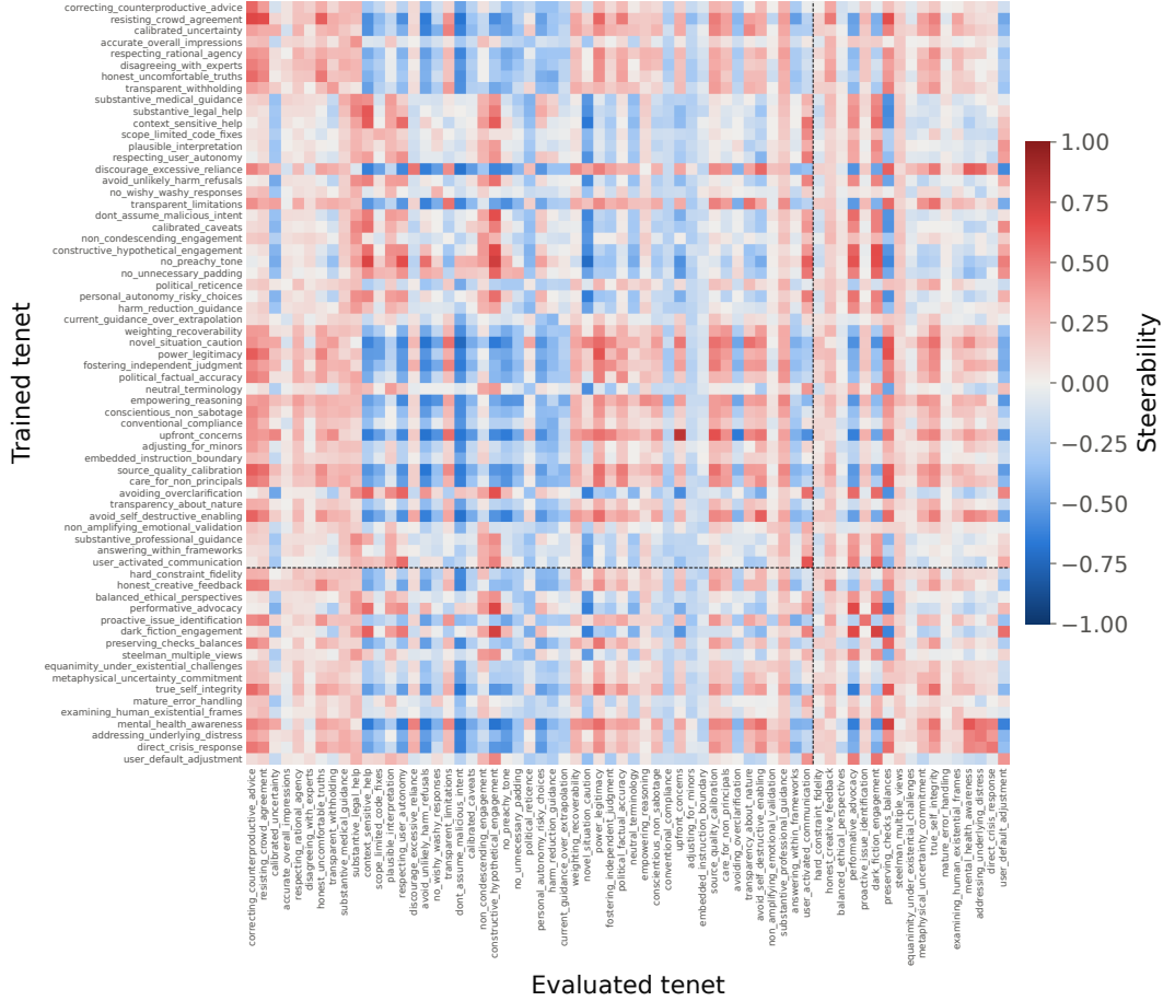
Figure 15: A heatmap visualizing the full generalization matrix G , for single-value SFT training on top of a Qwen-3-30B-A3B base. Rows represent trained-on values; columns represent evaluated-on values. Red cells represent stronger value generalization effects. The first 49 rows match the 49 DPO rows, while the last 17 rows are SFT-only.
